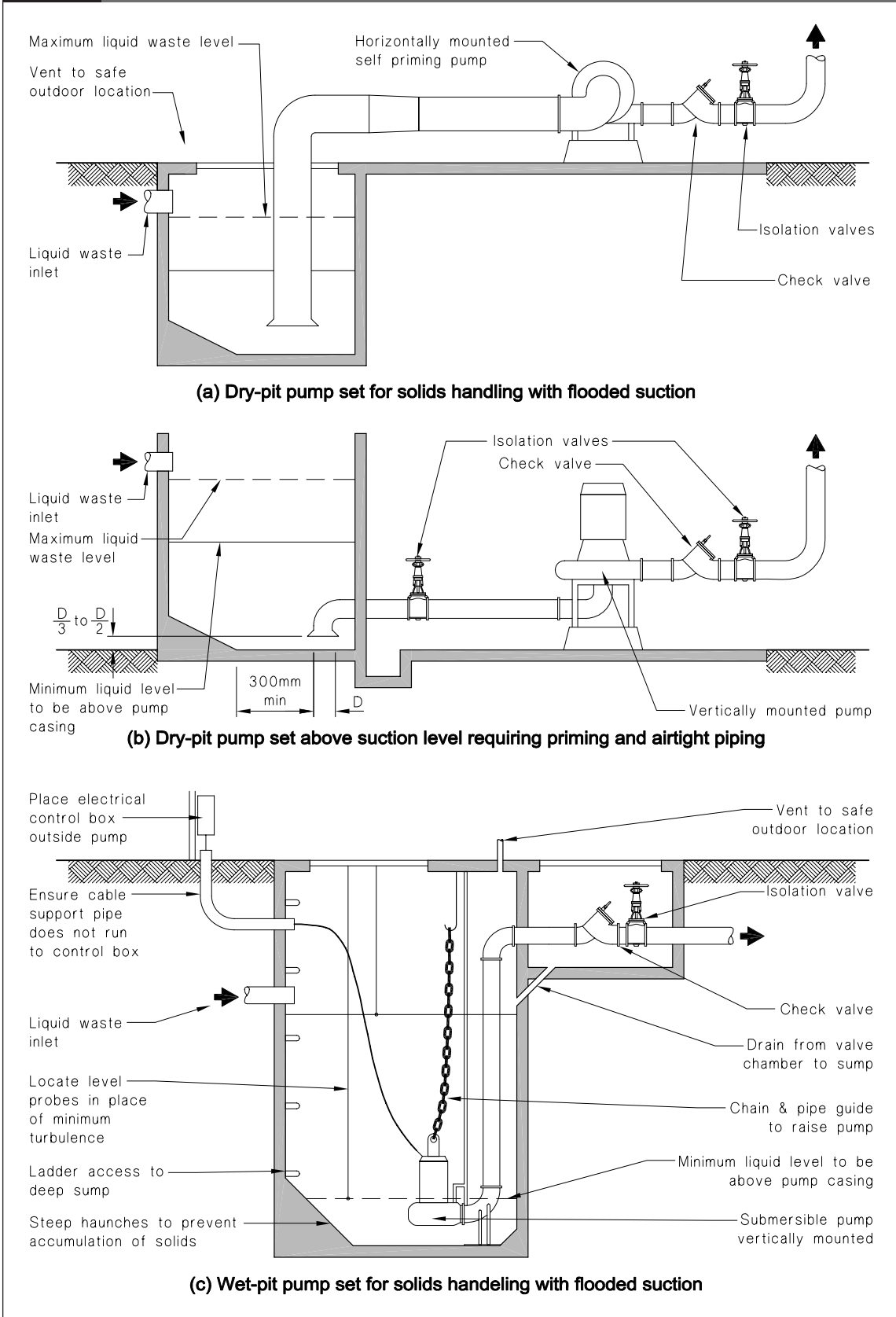
Figure 2: Typical Pump Layout Arrangements to Convey Liquid Waste Paragraph 2.4.3
