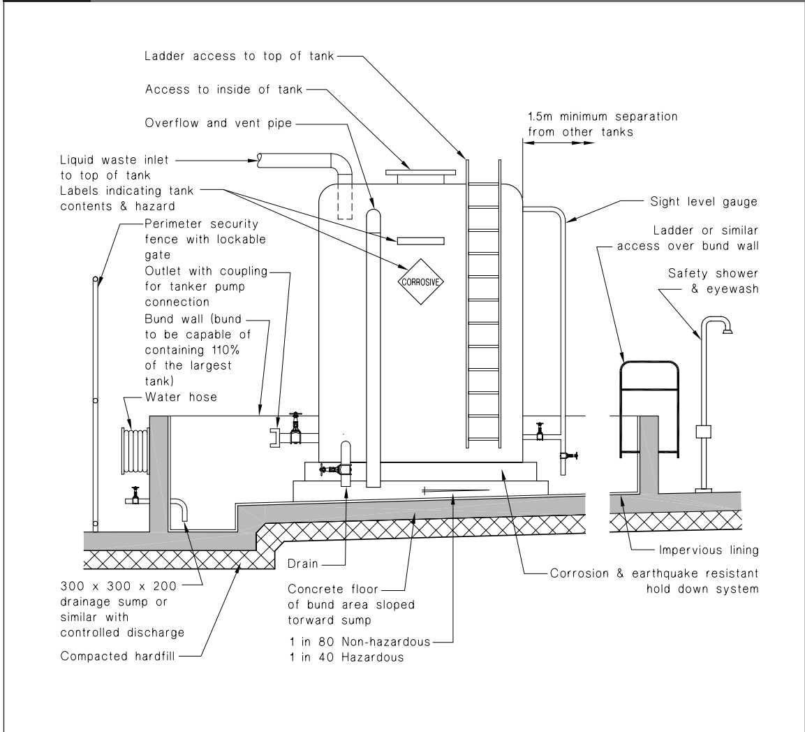
Figure 3: Typical Tank Storage Facility for a Corrosive Liquid Waste Paragraph 3.1.5
