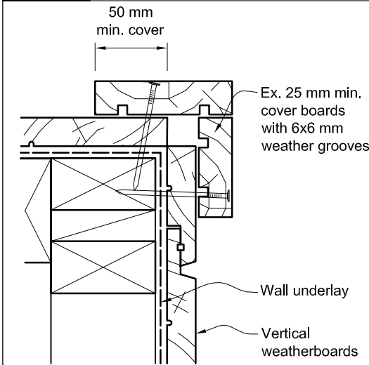
Figure 80: External corners for vertical weatherboards Paragraph 9.4.5.3
