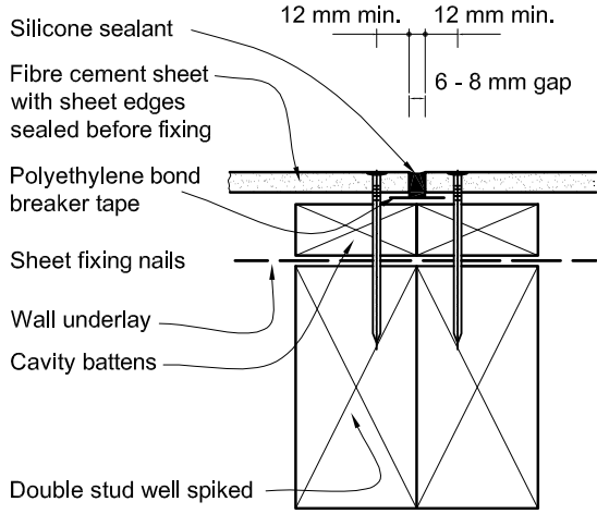
(a) SHEET JUNCTION CAVITY FIX
