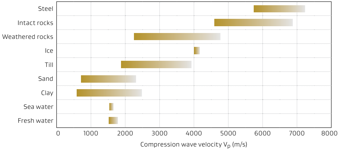
Figure 3.12: Representative P-Wave Velocities of Various Materials (from FHWA publication number FHWA NHI-01-031)
