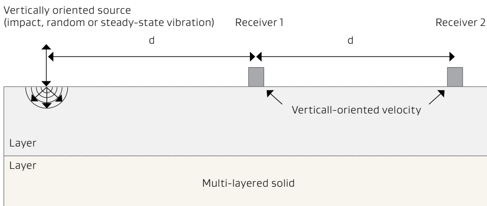
Figure 3.14: 2-Receiver Field Setup for Performing SASW Testing
