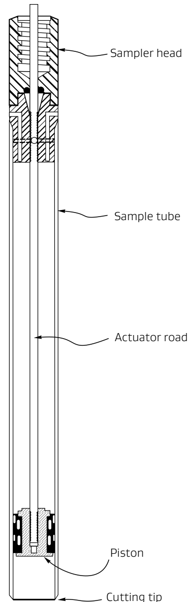
Figure 3.8: Schematic of Piston Sampler (after ASTM D 4700)
