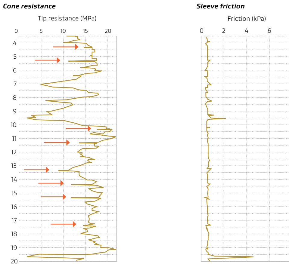
Figure B.5: multiple instances of rod changes in a CPT profile
