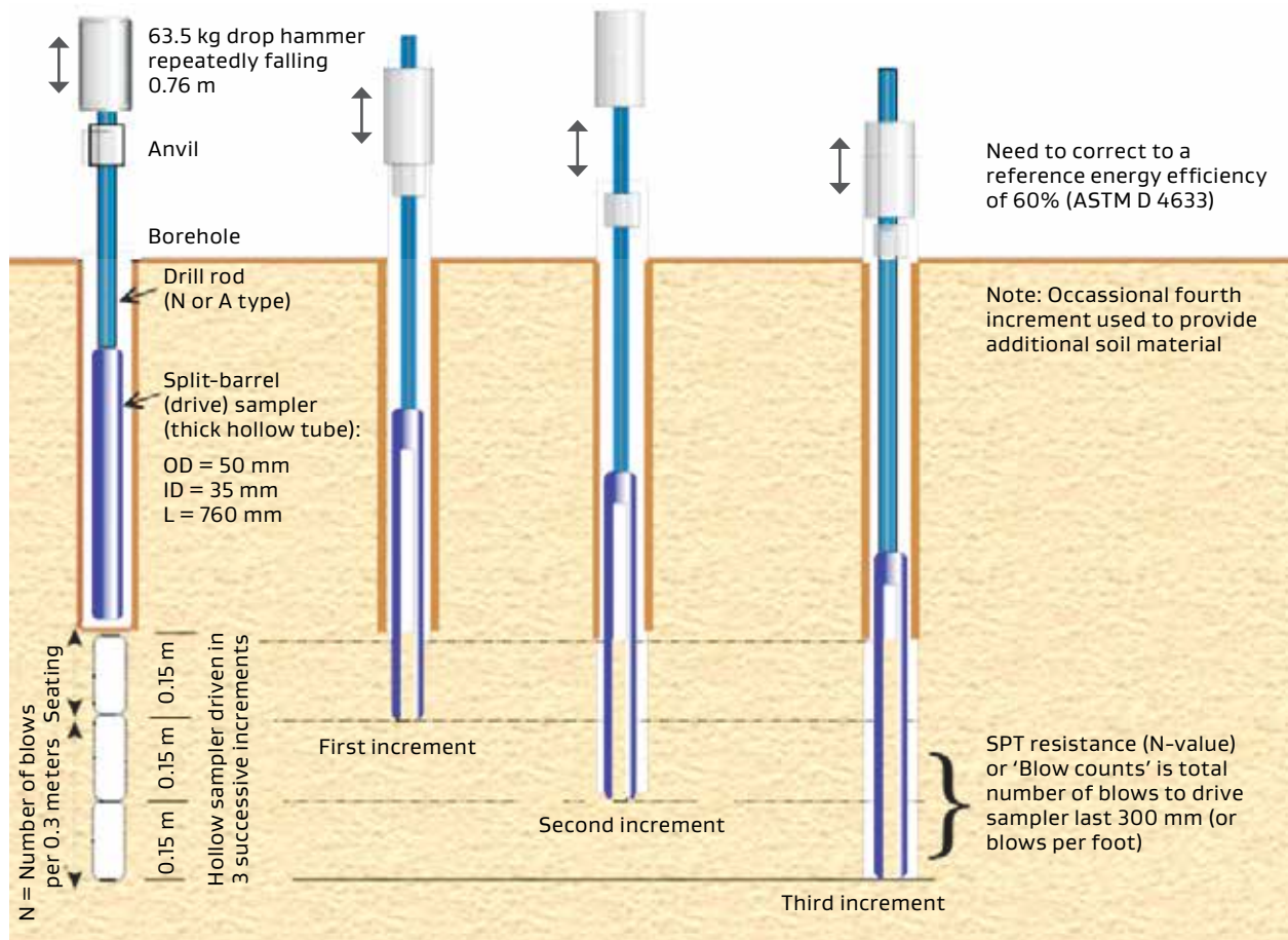
Figure 3.10: Sequence of Driving Sampler during Standard Penetration Test
