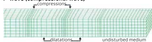
Figure 3.11: Particle Displacements with the Passage of P- and S-Waves
