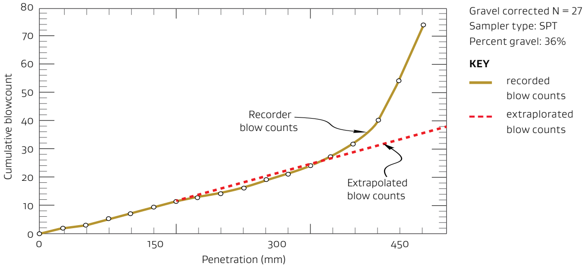
Figure D.2: Refusal penetration records
