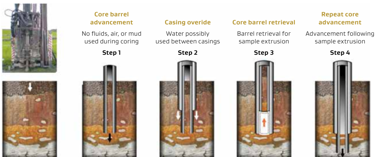
Figure 3.3: Typical Sonic Drilling Sequence
