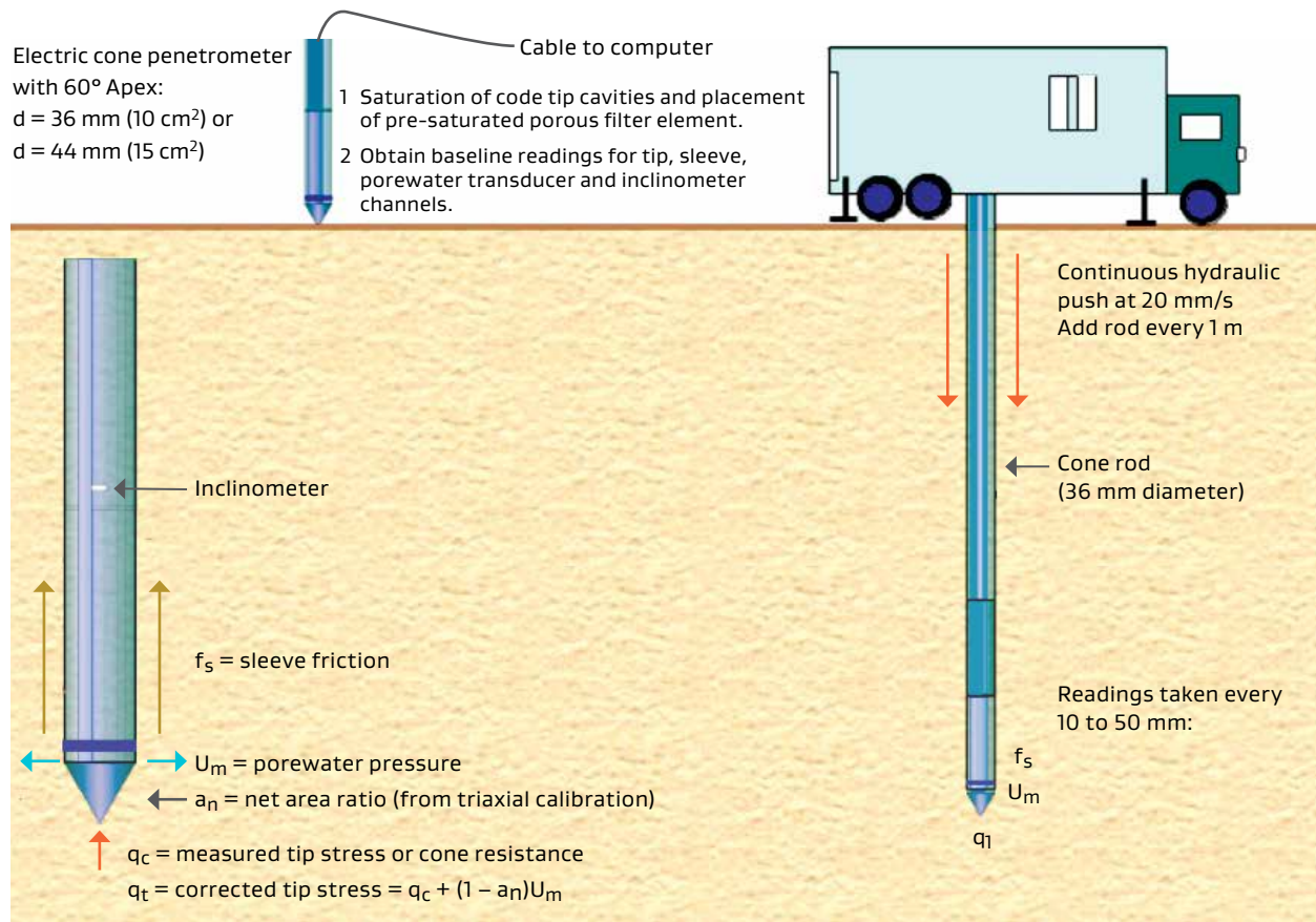
Figure 3: Procedures and Components of the Cone Penetration Test (from FHWA report NHI-01-031)
