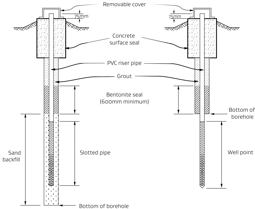
Figure 3.19: Typical Details of Observation Well Installations
