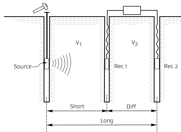
Figure 3.18: Crosshole Shear Wave Velocity Test Set-up
