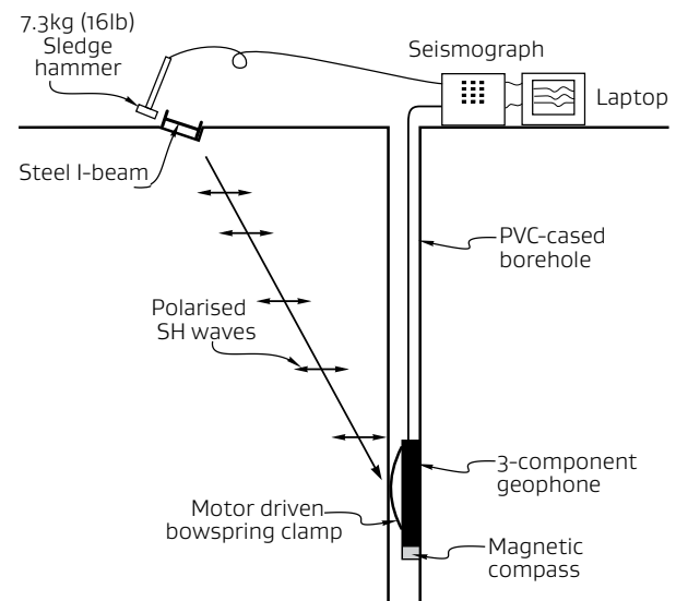
Figure 3.17: Downhole VSP Configuration for Polarised S-Wave Measurement
