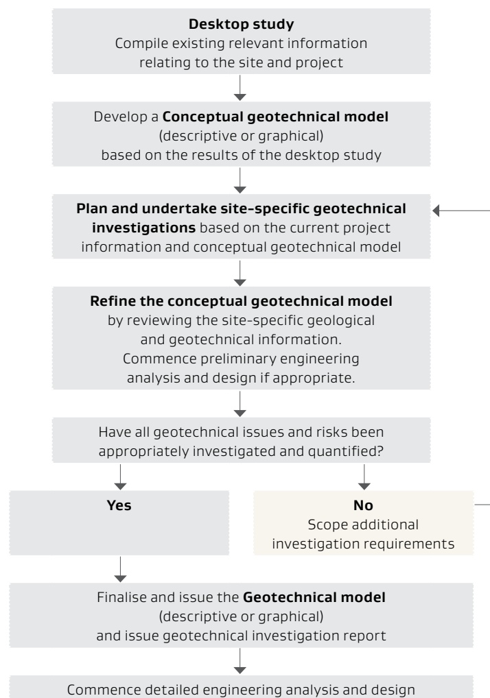
Figure 2: The Geotechnical Investigation Process
