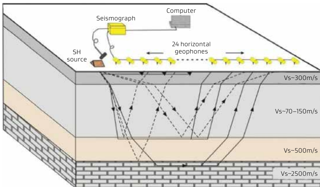
Figure 3.16: Schematic of Seismic Refraction Array and S-Wave Travel Paths
