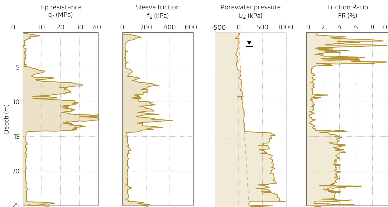
Figure 3.1: CPTu results from site in Christchurch near Avon River
