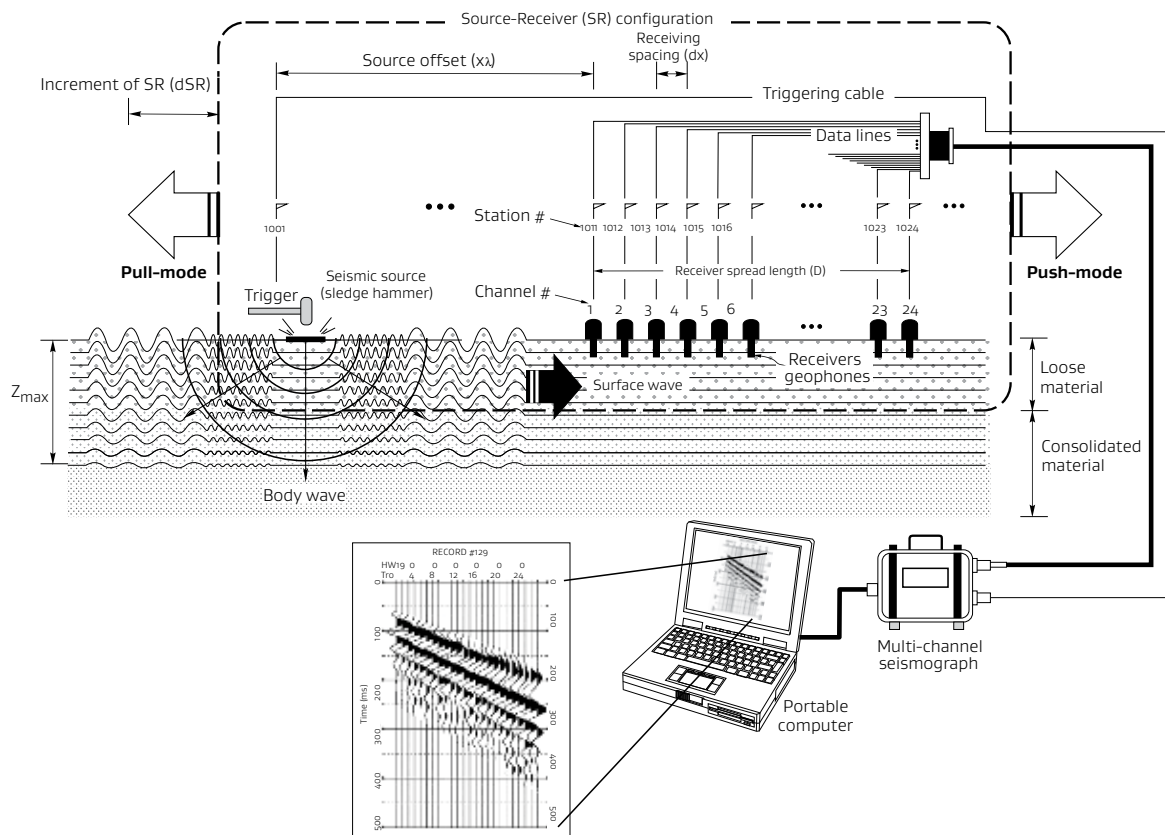
Figure 3.15: Field Setup for Performing MASW Testing (adapted from Park Seismic LLC)
