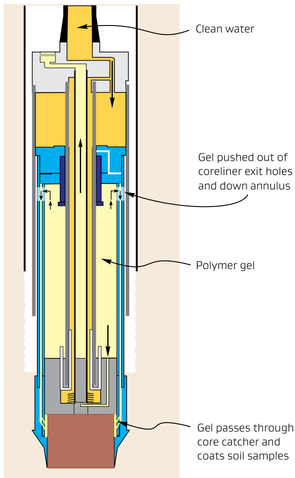
Figure 3.9: Schematic of GP-S
