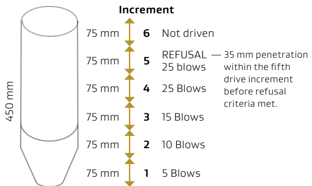
Figure D.2: Refusal penetration records
