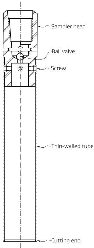
Figure 3.7: Schematic of Thin-Walled Shelby Tube (after ASTM D 4700)
