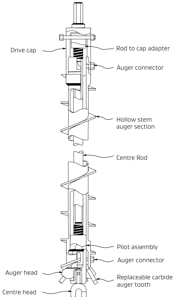
Figure 3.4: Typical Hollow-Stem Auger Components (ASTM D 4700)
