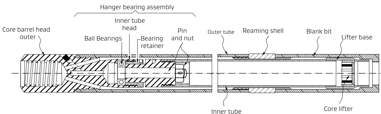
Figure 3.2: Swivel-Type Double Tube Core Barrel
