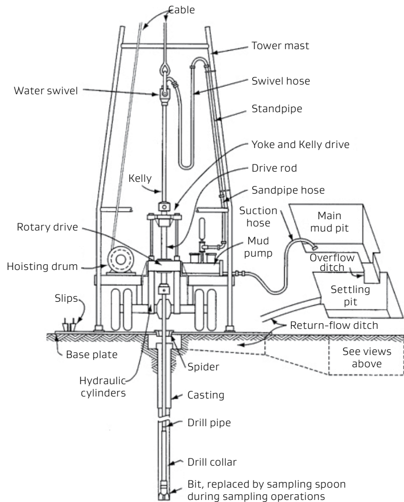
Figure 3.5: Rotary Wash Drilling (FHWA)
